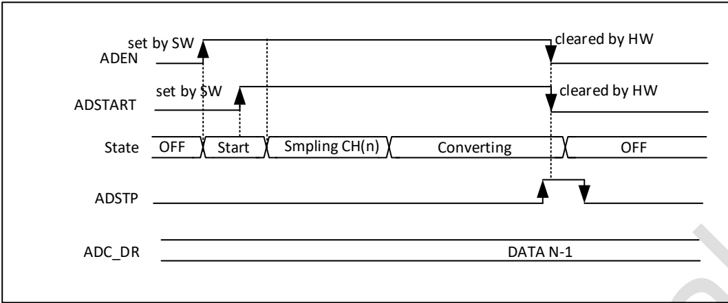
图 13-5 Stop timing
