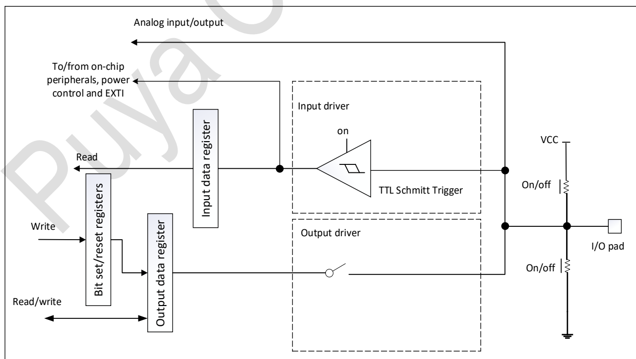
图 9-2 input floating/pull up/pull down configurations
